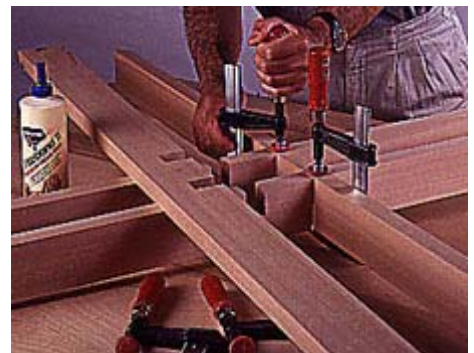
9 Glue and clamp together the half-lapped rail assembly. Check that the parts are square to one another.
